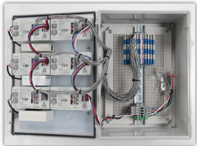
INSTALLER'S VIEW
